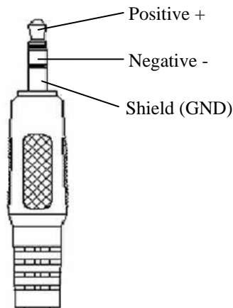
Balanced 3.5mm Connector
