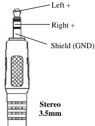
Stereo 3.5mm Connector
